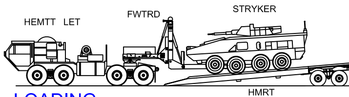
LOADING
